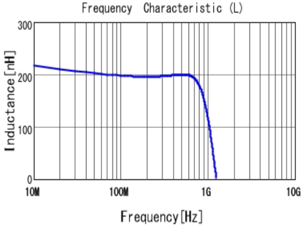
■ LQW18CAR21J00 L
