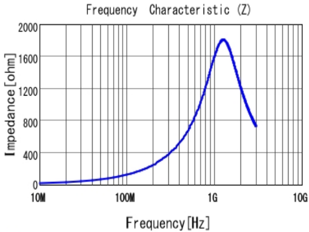
■ LQW18CAR21J00 |Z|
