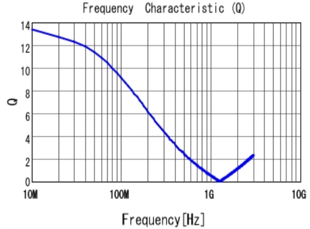
■ LQW18CAR21J00 Q
