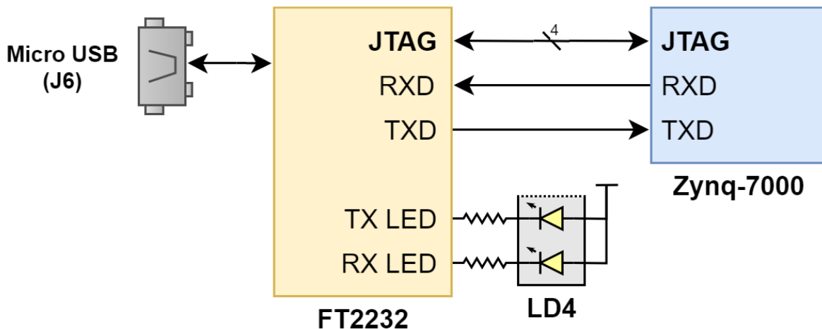
Figure 7.1: UART Connections
