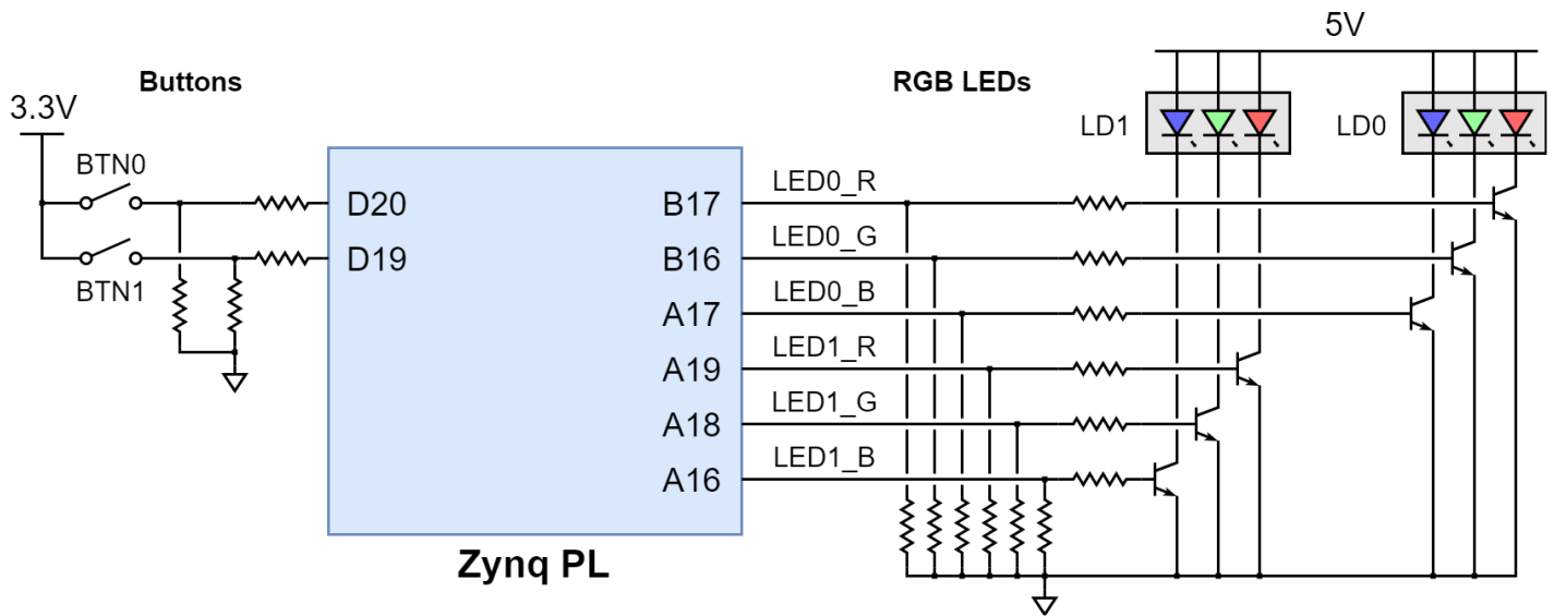
Figure 12.1: Eclipse Z7 Basic I/O
