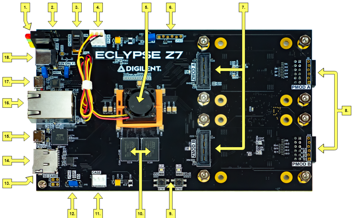
( https://digilent.com/reference/_detail/reference/programmable-logic/eclipse-z7/reference-manual/eclipse-callout.png?id=programmable-logic%3Aeclipse-z7%3Areference-manual ) Eclipse Z7 Callout Diagram
