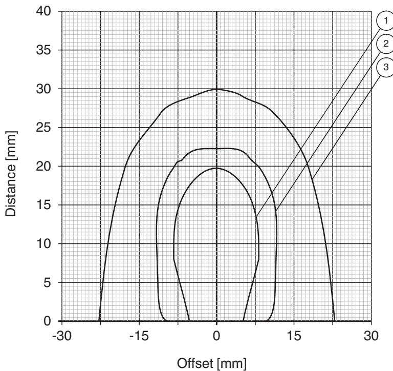
Reading range in air IQC35-10
