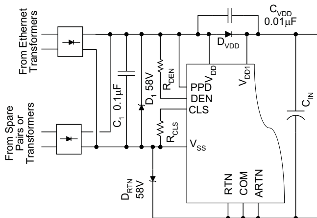
Figure 24. Example of Added ESD Protection for PoE Priority
