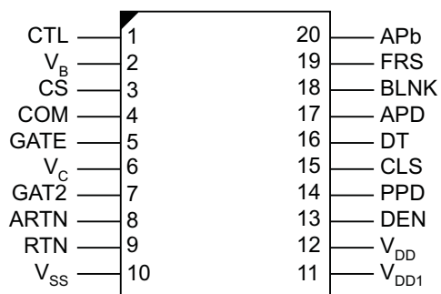
PWP PACKAGE (TOP VIEW)
