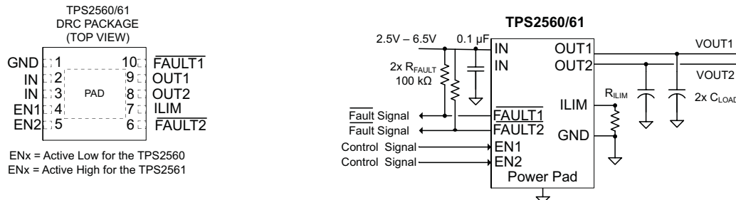
Figure 1. Typical Application as USB Power Switch
