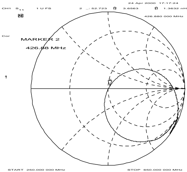
Smith Chart
