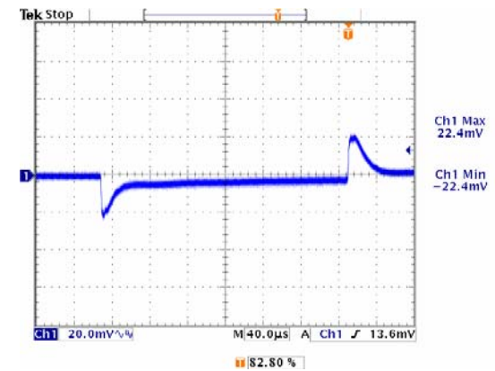
Figure 23: Transient response, 1.2V /20A, Ch1: Vo
