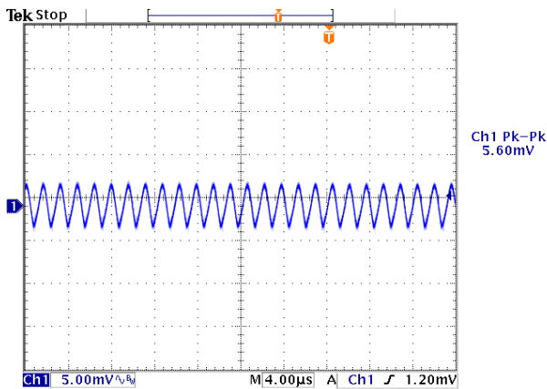
Figure 11: Output ripple & noise at 12Vin, 1.2V/20A out
