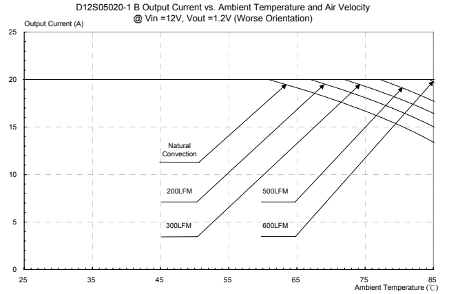
Figure 37: Output current vs. ambient temperature and air velocity @ Vin=12V, Vout=1.2V (Worst Orientation)
