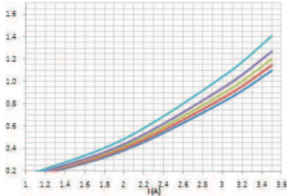
Figure 35. Buck 1 Losses (W) vs Output Current V_{IN} = 12\text{ V} , f_{SW} = 500\text{ kHz}
