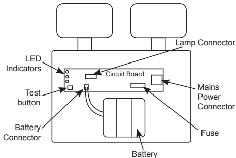
Fig 2. Internal Layout
