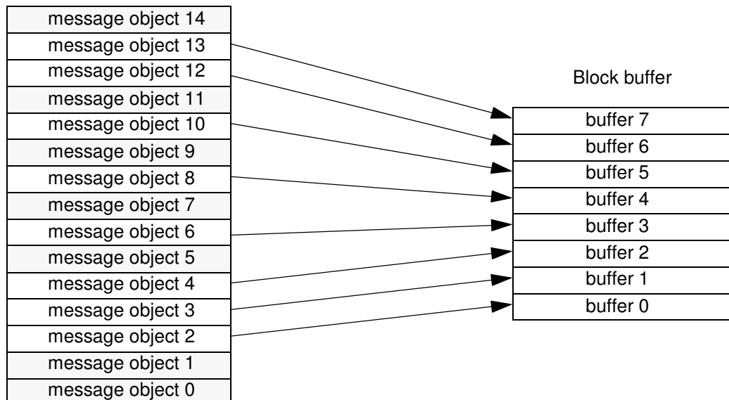
Figure 49. Buffer mode
