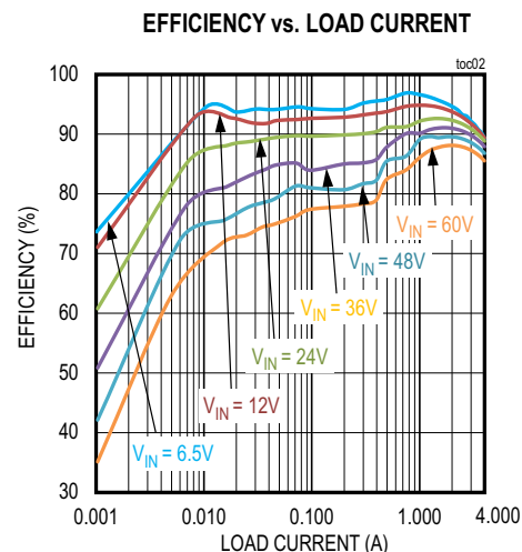
CONDITIONS: 5V OUTPUT, PFM MODE, f_{SW} = 350kHz
