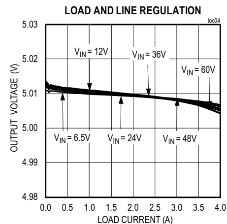
CONDITIONS: 5V OUTPUT, PWM MODE
