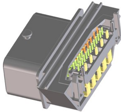
CMC 28WAY Header
