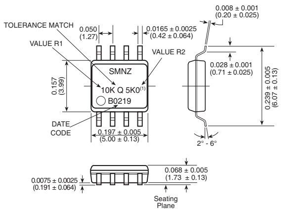
FIGURE 3 - DIMENSIONS AND IMPRINTING EXAMPLE in inches (millimeters)
