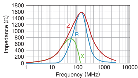
MMZ1608Y152BTD25
