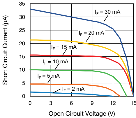
Fig. 1 - Short Circuit Current vs. Open Circuit Voltage
