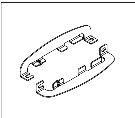
Fig. 23-2 ZM10.Wall Wall mounting bracket*)
