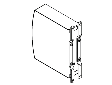
Fig. 23-2 Wall mounting with DIN rail brackets*)
