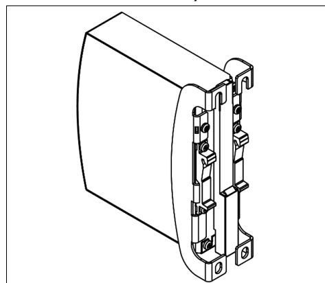
Fig. 23-4 Side mounting with DIN rail brackets*)
