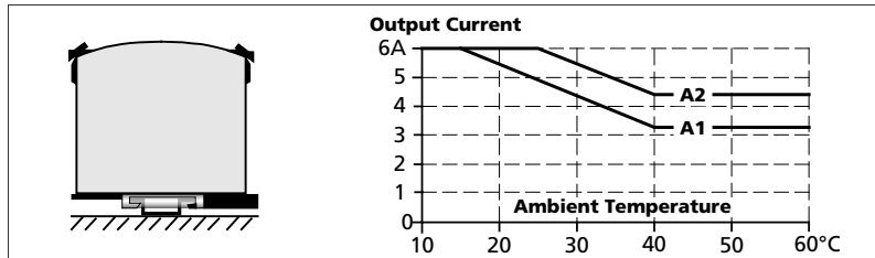
Fig. 24-8 Mounting Orientation C (Table-top mounting)
