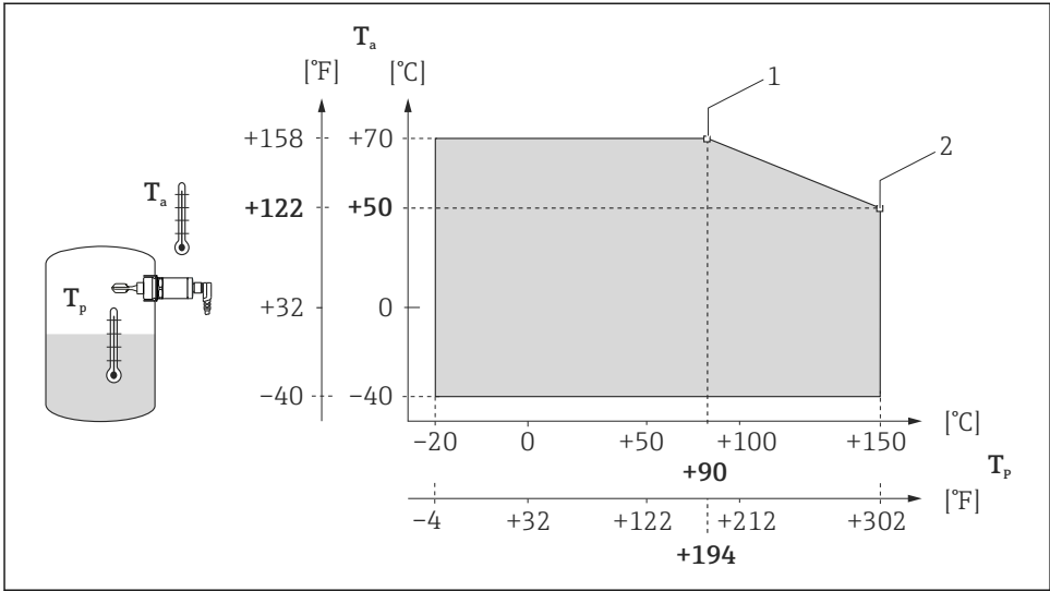
18 Derating curve: 150 °C (302 °F)
