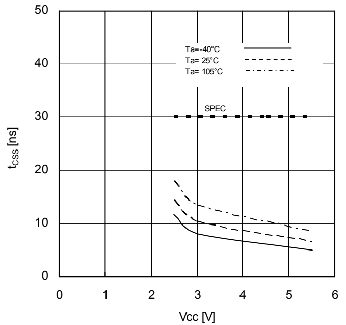
Figure 19. CSB Setup Time vs Supply Voltage
