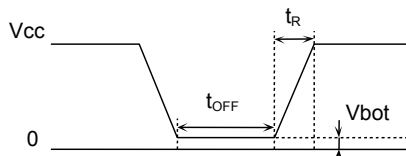
Figure 55. Rise waveform
