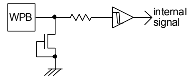
Figure 52. WPB input equivalent circuit
