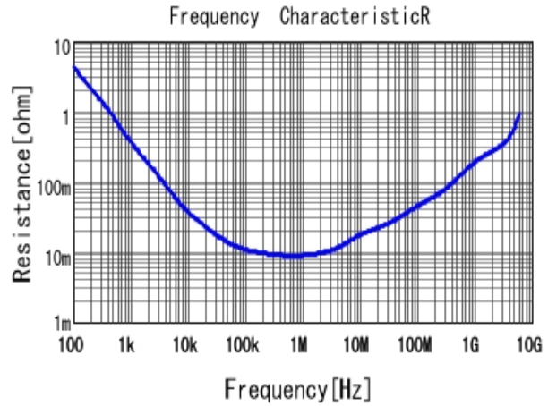
■ GRT155C80J475ME13 R DCOV, 25degC
