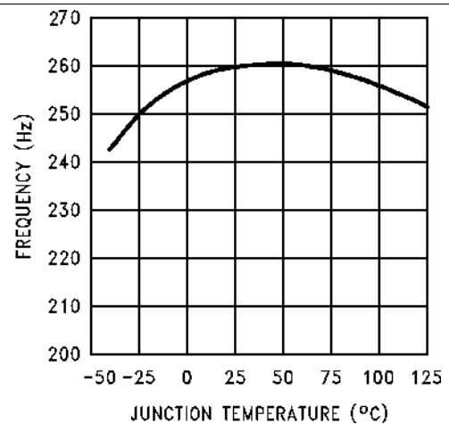
Figure 10. Switching Frequency
