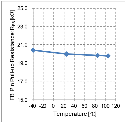
Figure 22. FB Pin Pull-up Resistance vs Temperature
