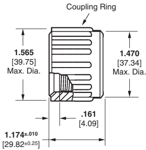
Coupling Ring
