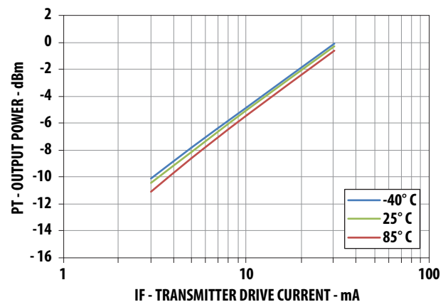
Figure 6. Typical optical output power vs. drive current
