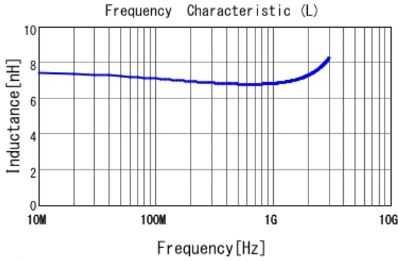
■ LQP03TN6N8J02 L
