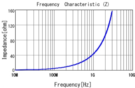
■ LQP03TN6N8J02 |Z|
