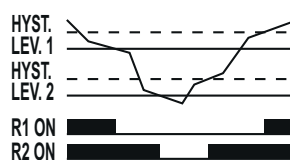
Fig. 1 Operation diagram
