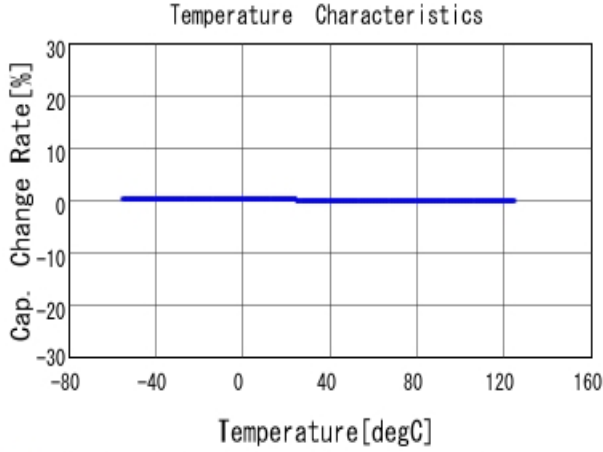
■ GRM0335C1E101FA01 C-Temp. capchange, DCOV, AC1Vrms
