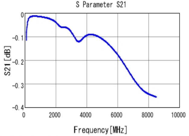
■ GRM0335C1E101FA01 S21 DCOV, 25degC
