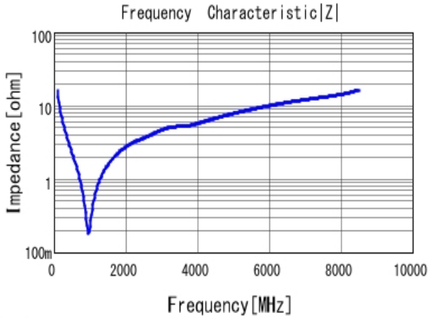
■ GRM0335C1E101FA01 |Z| DC0V, 25degC
