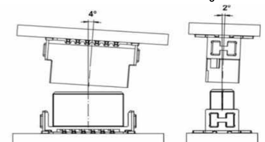
Admissible mismatching
