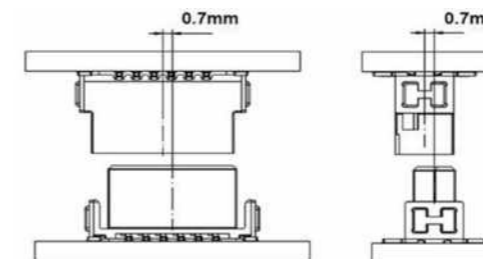
Admissible inclination
