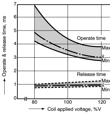
4.-(1) Operate & release time (without diode, 1a type)
