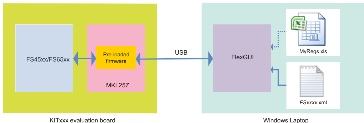
Figure 18. Software overview
