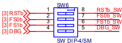
Figure 17. Switch SW6
