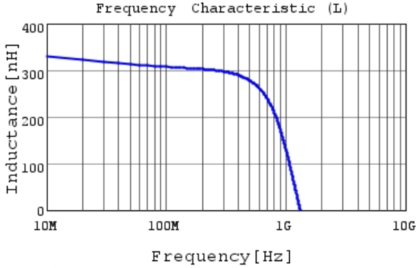
LQW18CNR33J0H L
