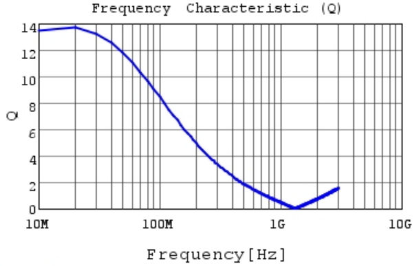
LQW18CNR33J0H Q
