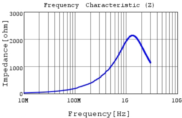
LQW18CNR33J0H |Z|
