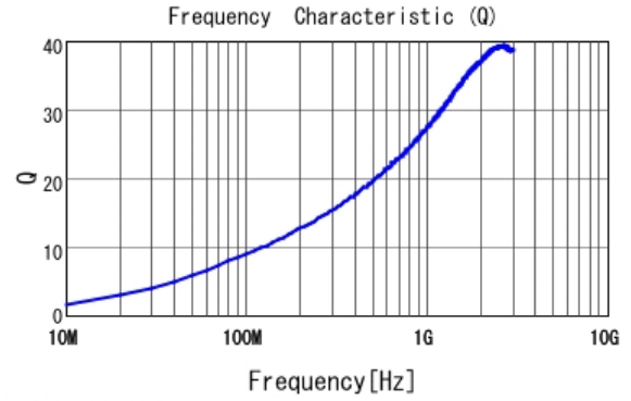
■ LQP03TN3N9C02 Q
