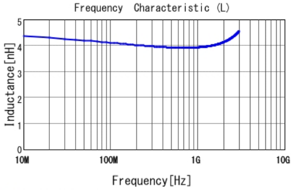
■ LQP03TN3N9C02 L
