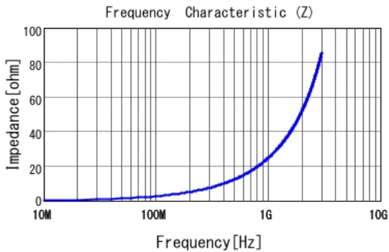
■ LQP03TN3N9C02 |Z|
