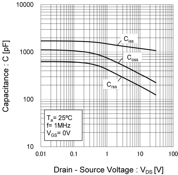
Fig.18 Typical Capacitances vs. Drain - Source Voltage
