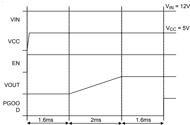
Figure 1. Start-Up Sequence
