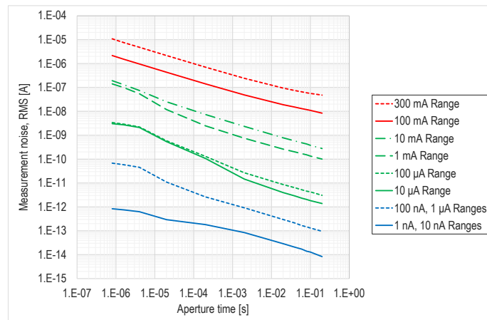
Figure 21. Current measurement noise
