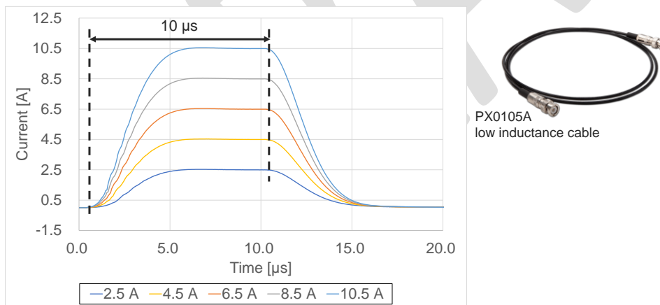
Figure 9. 10 \mu\text{s} narrow pulse output with measuring at 15 MSa/s sampling rate
