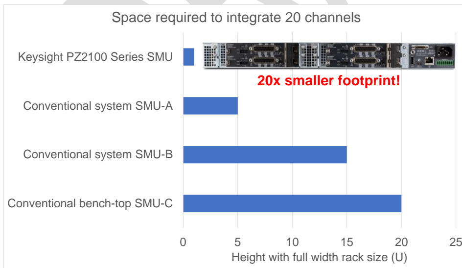
Figure 4. 20x higher channel density integrating 20 channels in 1 U height, full width, rack size
