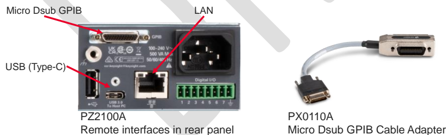
Figure 14. Remote interface in PZ2100A rear panel and PX0110A GPIB cable adapter
