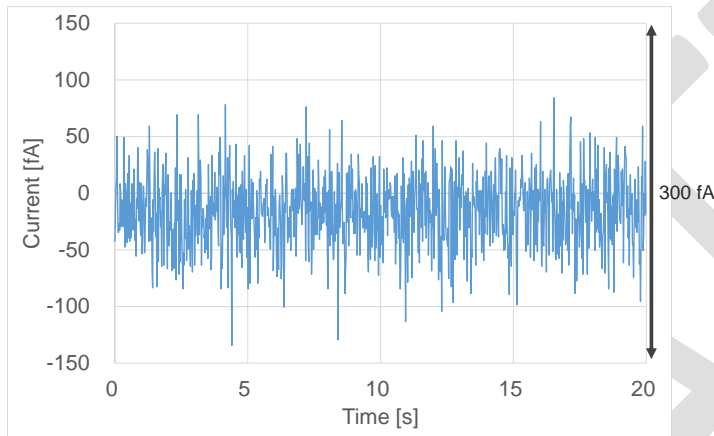
Figure 7. Measurement noise, 10 nA range, no load, 0 V, triax cable (3 m)
