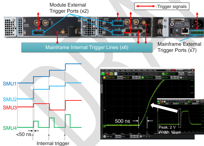
Figure 12. Internal trigger lines enabling channel synchronization at less than 50 ns accuracy and external trigger ports enabling synchronization with any external equipment
