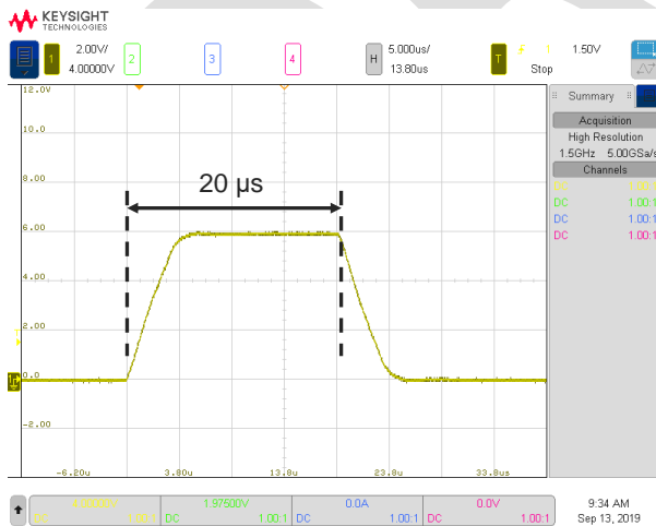
Figure 8. Narrow pulse down to 20 \mu s enables you to suppress self-heat effect to reveal the true characteristics of the devices
