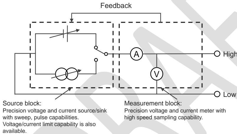
Figure 5. SMU simplified block diagram
