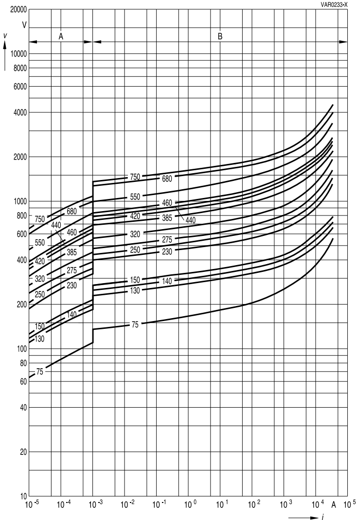
SIOV-B40K75 ... K750
