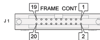
J1 Connector
