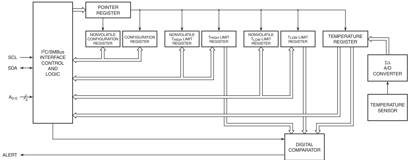
Figure 3-1. Block Diagram
