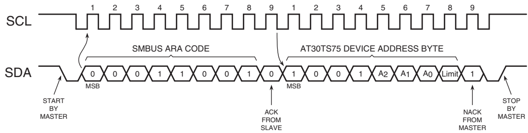
Figure 10-1. SMBus Alert
