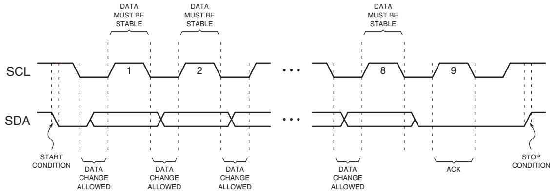
Figure 4-1. START, STOP, and ACK
