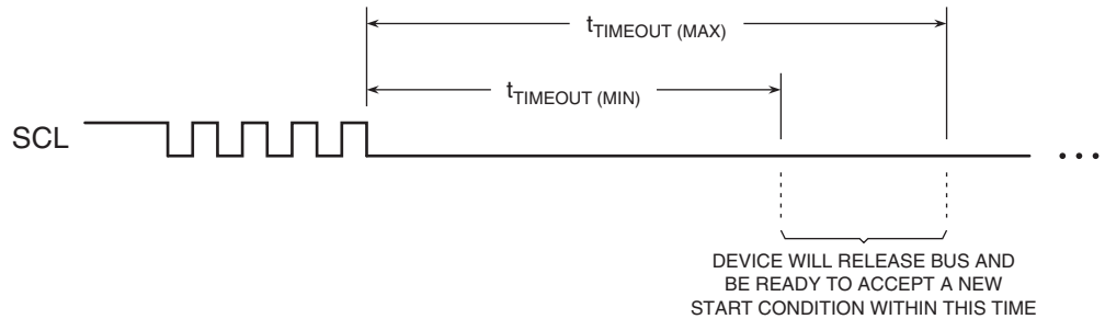
Figure 10-2. SMBus Timeout
