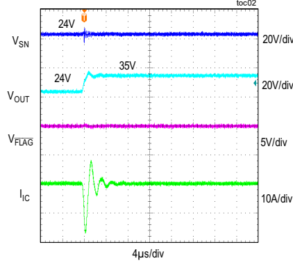
REVERSE-BLOCKING RESPONSE toc02
