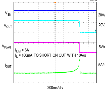
CURRENT-LIMIT RESPONSE toc05
