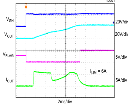
POWER-UP RESPONSE WITH 2200 \mu F CAPACITOR AT NO LOAD toc01
