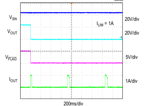
AUTORETRY CURRENT-LIMIT RESPONSE toc06
