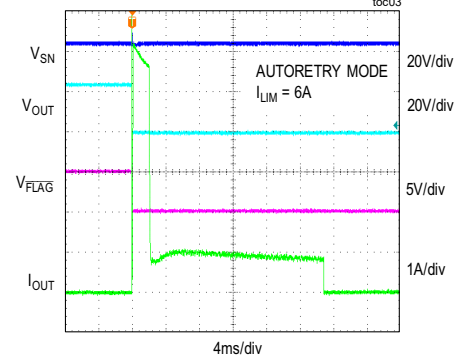
THERMAL FOLDBACK DUE TO OUTPUT SHORT-CIRCUIT toc03
