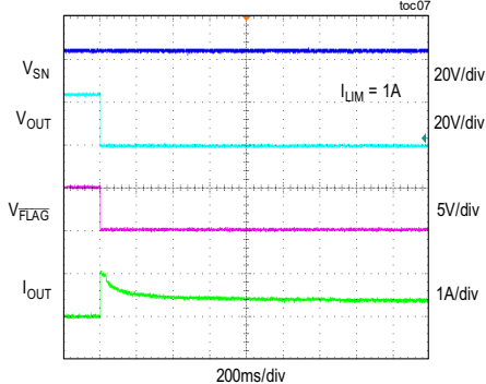
CONTINUOUS CURRENT-LIMIT RESPONSE toc07
