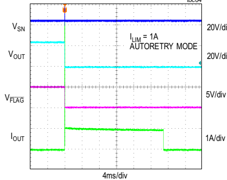
OUTPUT SHORT-CIRCUIT RESPONSE toc04
