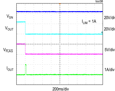
LATCH-OFF CURRENT-LIMIT RESPONSE toc08
