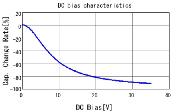
■ GRT31CR6YA106KE01 C-DC bias capchange, 25.0degC, AC1.
