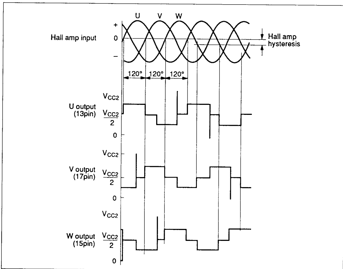
Figure 4 Timing Chart
