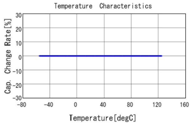
■ GRM31C5C3A102JWA3 C-Temp. capchange, DCOV, AC1Vrms
