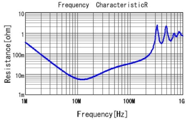
■ GRM31C5C3A102JWA3 R DCOV, 25degC
