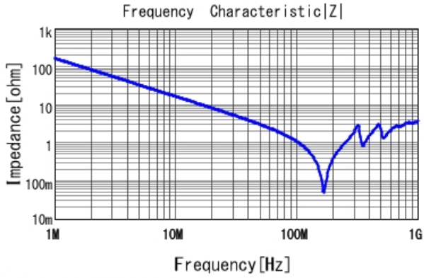
■ GRM31C5C3A102JWA3 |Z| DCOV, 25degC
