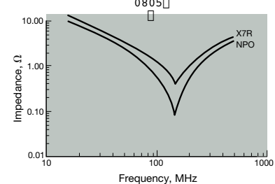
Variation of Impedance with Ceramic Form Impedance vs. Frequency 1000 pF - COG (NP0) vs X7R 0805
