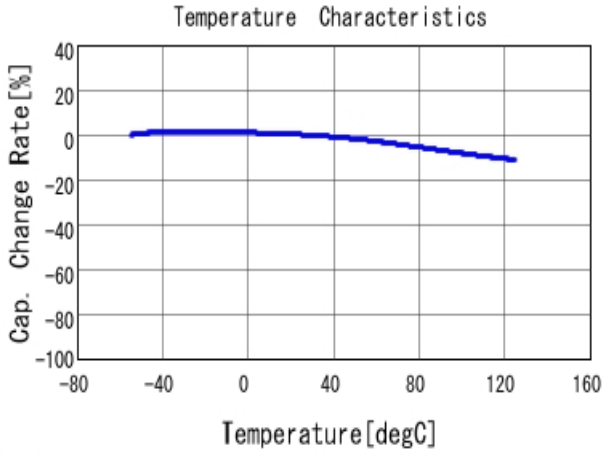
■ KCM55WR71H336MH01 C-Temp. capchange, DCOV, ACO, 5Vrms
