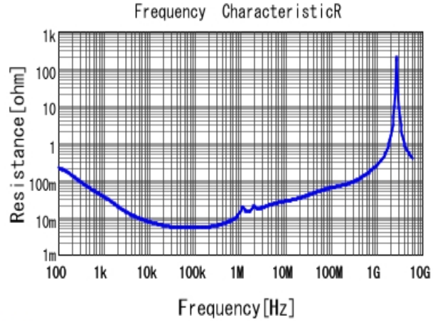
■ KCM55WR71H336MH01 R DCOV, 25degC
