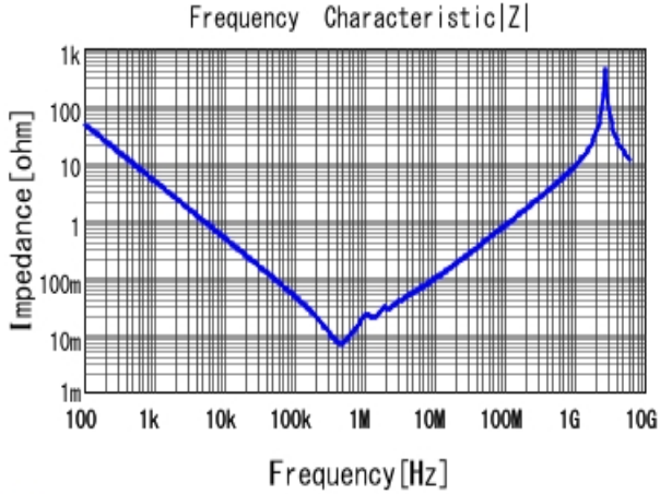
■ KCM55WR71H336MH01 |Z| DCOV, 25degC
