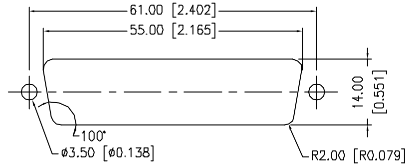
PANEL CUTOUT
