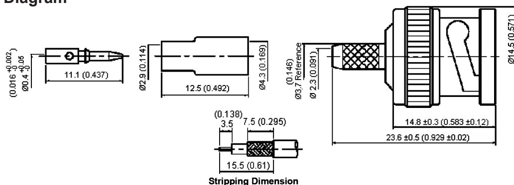
Stripping Dimension
