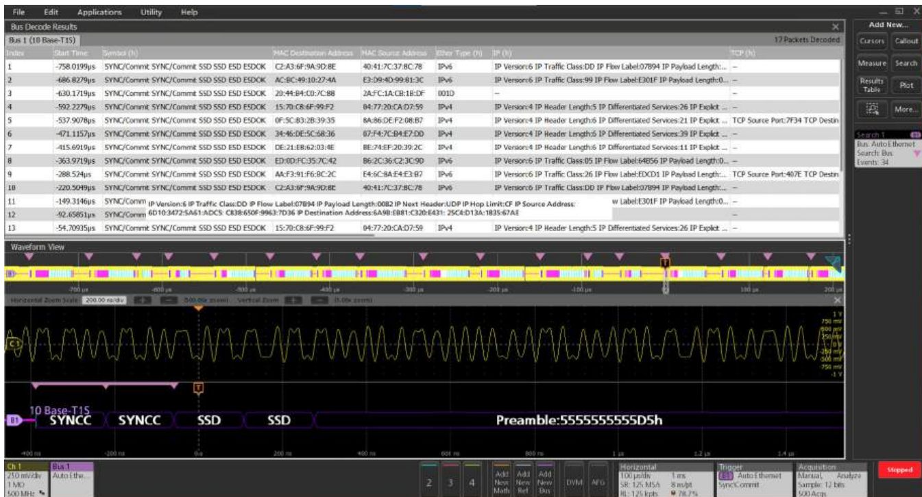
10BASE-T1S bus decode and results table in a tabular format. Searching the 10BASE-T1S bus decode with search on Sync/Commit with 34 occurrences shown on the search badge.
