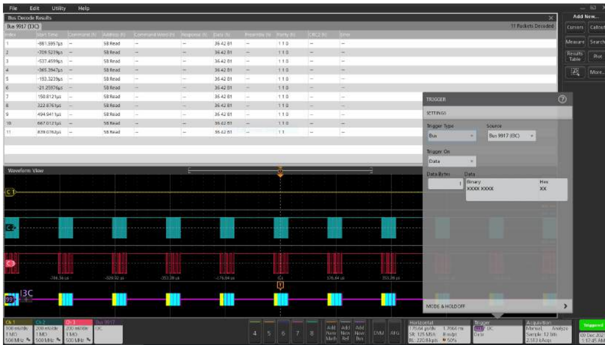
Triggering on a specific 7-Bit read address value on the I2C bus.
