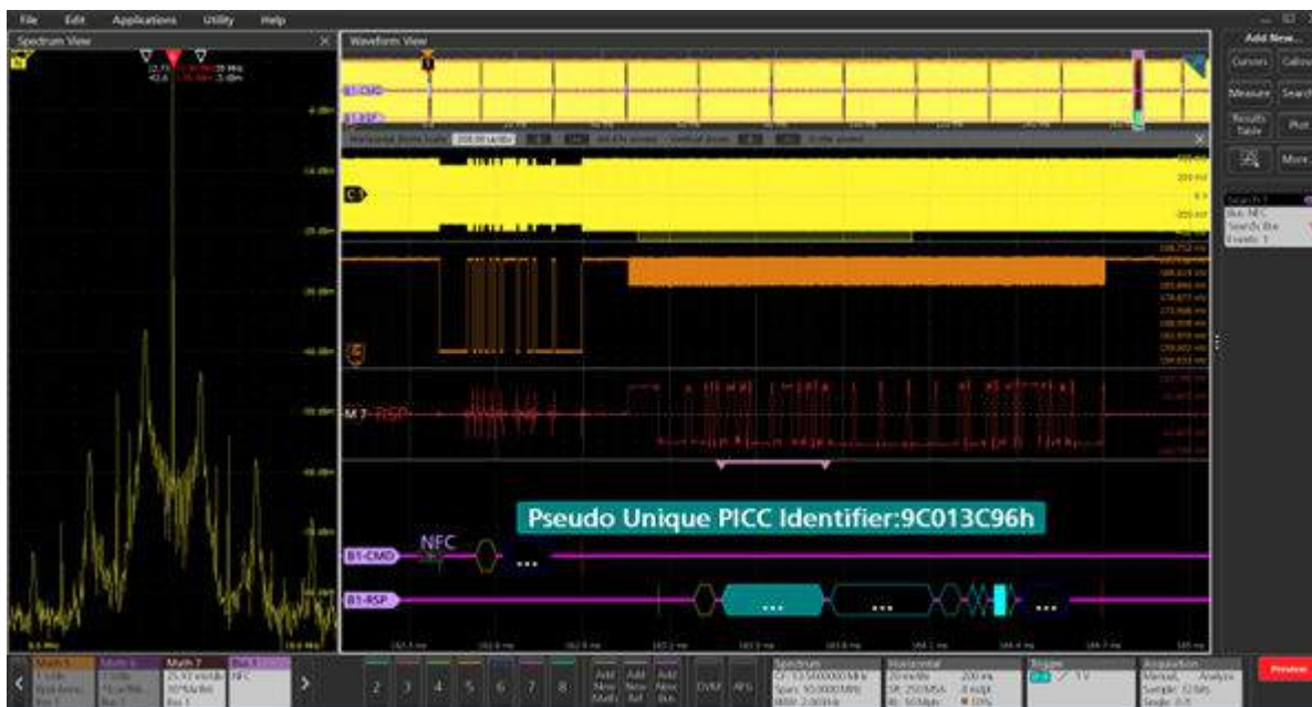
NFC Search for PUPI
