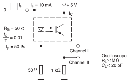
Figure 4. Test circuit, saturated operation
