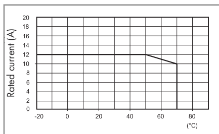
L 96 - Rated current vs ambient temperature
