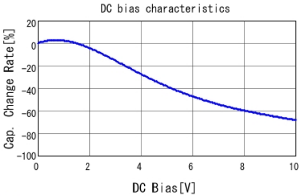
GCM32EC71A476KE02 C-DC bias capchange, 25.0degC, AC0.
