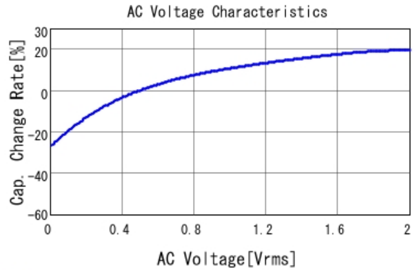
GCM32EC71A476KE02 C-AC Voltage capchange, DC0V, 25.0d
