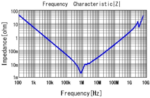
GCM32EC71A476KE02 |Z| DC0V, 25degC
