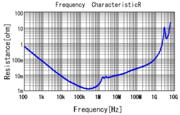
GCM32EC71A476KE02 R DC0V, 25degC
