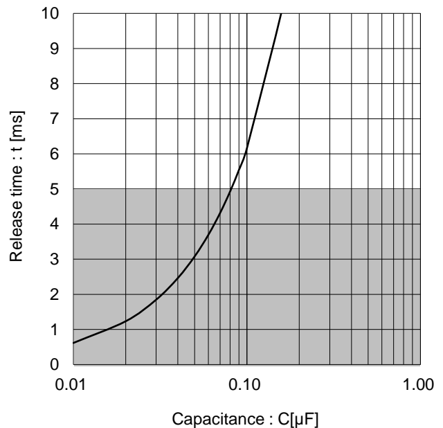
Figure 9. Release Time (Reference Data @R=100kΩ)
