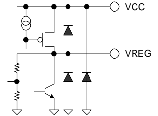
Figure 53. VREG, VCC
